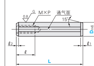
MSTM (带拉拔螺纹m6型)
